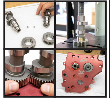
D Install front cam .100" thick thrust washer & retaining clip. Install clip with sharp ID edge outward.
