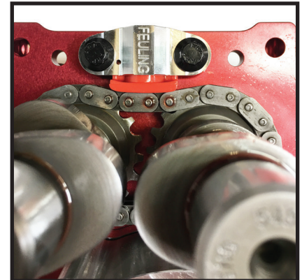
Make sure tensioner pad is square to the chain & the pad moves up & down.
