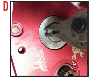
D Install front cam .100" thick thrust washer & retaining clip. Install clip with sharp ID edge outward.
