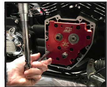
Rotate the engine several more times and final torque to 90-120 in/lbs .
