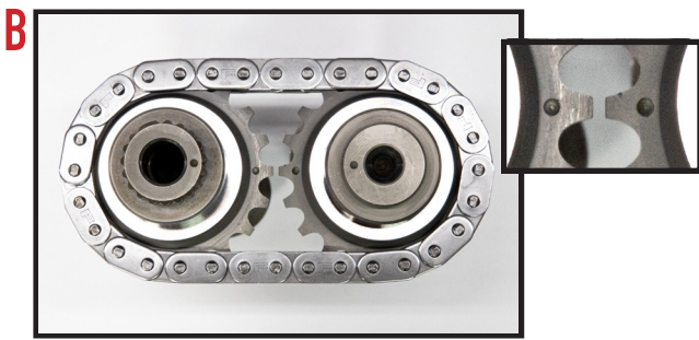
B Install chain on the cams & verify that the timing marks are aligned.
