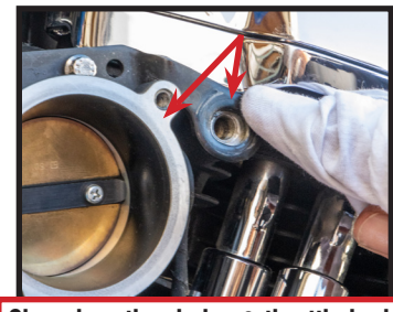
Clean breather holes & throttle body surfaces
