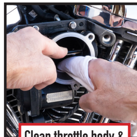
Clean throttle body & blade.
