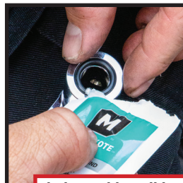
Lube and install inner and outer breather O-rings, use with O-ring lube.
